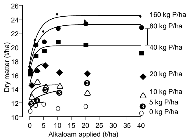
Figure 3. The effect of Alkaloam™ and P fertiliser on yield totalled for all four years of the trial. Not all of the fertiliser application rates could be adequately fitted to the growth curve (Mitscherlich). The error bar shows the significant differences ( P > 0.05 ) between the means (symbols) (from Summers et al. , 2001).
