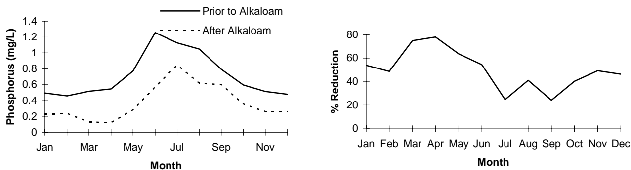
Figure 1. a) Monthly P concentrations - Meredith Drain, b) Monthly % P reductions - Meredith Drain after Alkaloam™ amendment (From Rivers, 1996).
